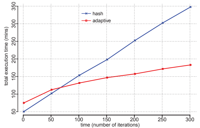
Figure 9. Cumulative execution time after expanding the heart cell FEM using a forest fire model (extra 10^7 vertices and 3 \cdot 10^7 edges). Results were obtained in a cluster of 63 workers (64GB RAM, 10GbE and 12 Cores)
