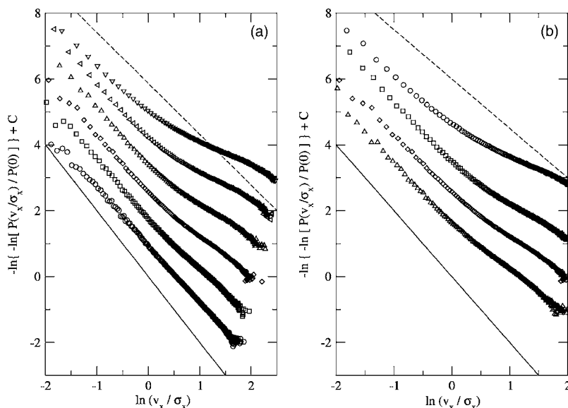
FIG. 8. Boundary heating. (a) -\ln\{-\ln[P(v_x/\sigma_x)]\} vs \ln(v_x/\sigma_x) for N=350 , \phi=0.02 and \eta=0.9 ( \circ ), 0.8 ( \square ), 0.7 ( \diamond ), 0.6 ( \triangle ), 0.5 ( \nabla ), and 0.4 ( \nabla ). (b) -\ln\{-\ln[P(v_x/\sigma_x)]\} vs \ln(v_x/\sigma_x) for N=350 , \eta=0.7 and \phi=0.01 ( \circ ), 0.02 ( \square ), 0.03 ( \diamond ), and 0.05 ( \triangle ).
