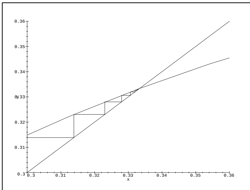
Fig. 6. a = 1.5 , ingezoomed.
