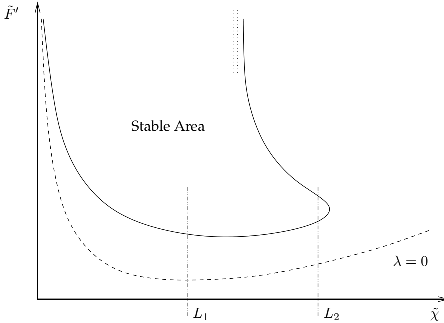
Figure 5.9: General picture of stability in the plane (\tilde{x}, \tilde{F}')
