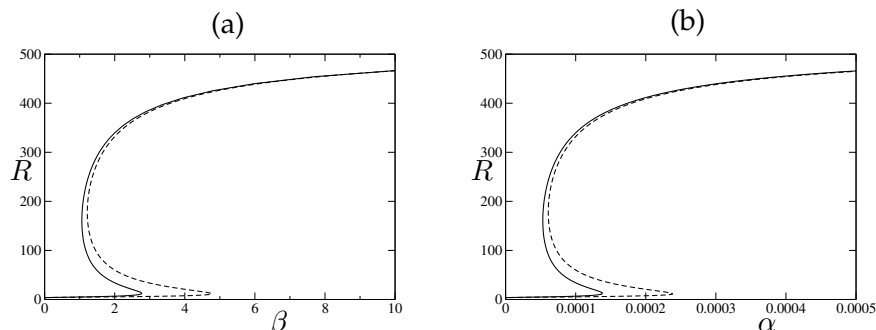
Figure 2.6: Comparison between the nonlinear problem (solid line) and the linearized one (dashed line) with (a) \beta and (b) \alpha as the bifurcation parameter.
