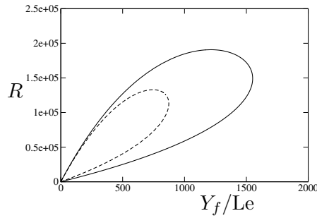
Figure 2.9: The global picture of the (Y_f/Le, R) bifurcation diagram. Note that there is a branch of solutions (almost) coinciding with the horizontal axis.
