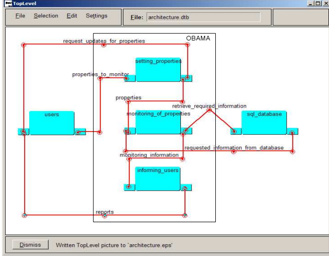
Figure 1. Agent Architecture
