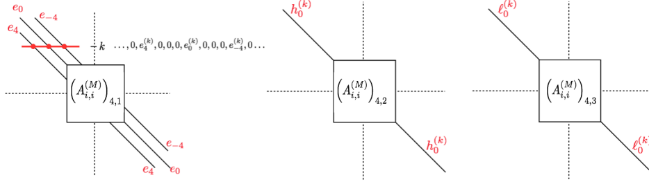
Figure 7: Structure of the components of the operator A_{i,i} . The infinite dimensional diagonal and tridiagonal terms are defined so that the composition AA^\dagger acts as the identity out of \Pi^{(M+4)}X .
