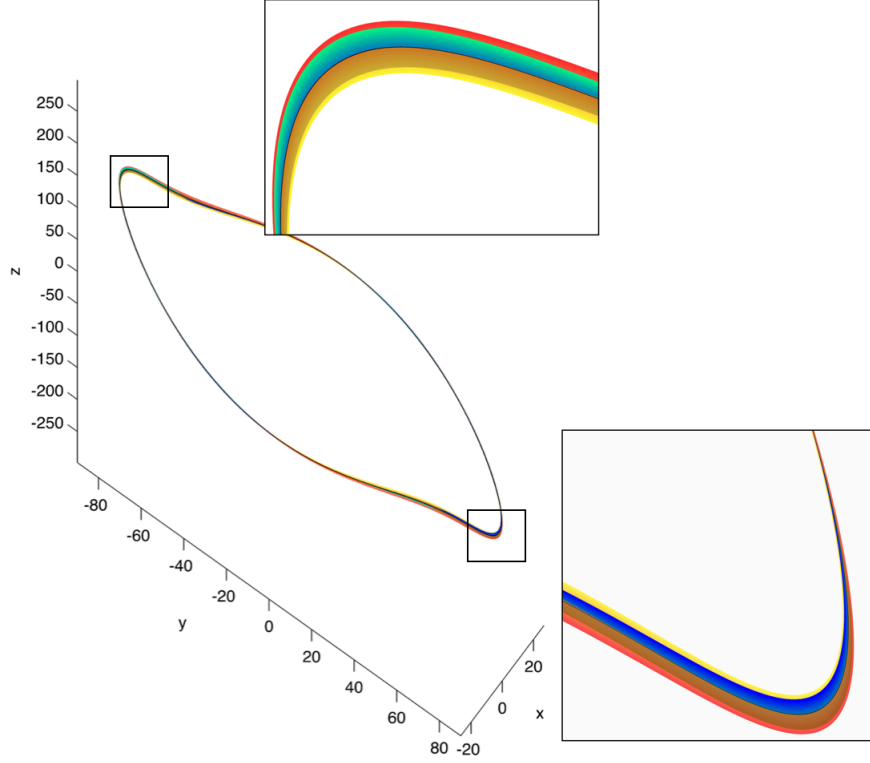
Figure 5: Image of the parameterization of two submanifolds of the local stable manifold associated to the periodic orbit \Gamma(t) . Only the first three components of P_N(w, z) are drawn. The red-to-yellow surface is the image of the submanifold tangent to the eigenspace a_{(1,0)}(w) , associated to the Floquet exponent \lambda_1 \approx -7 . The green-to-blue surface is the submanifold tangent to the eigenspace a_{(0,1)}(w) , associated to \lambda_2 \approx -8 .
