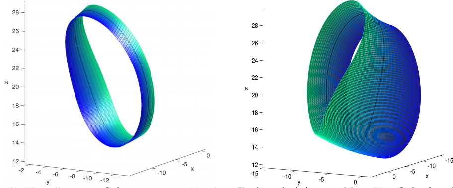
Figure 2: Two images of the parameterization P_N(w, z) , |z| \leq \nu , N = 10 , of the local stable manifold associated to the periodic orbit of the Lorenz system at parameter \rho = 22 . In the left case \nu = 1 and the N -tail norm is \|H\|_{r,\nu}^\infty \leq 1.024 \cdot 10^{-11} . On the right \nu = 4 and \|H\|_{r,\nu}^\infty \leq 9.77 \cdot 10^{-5} .
