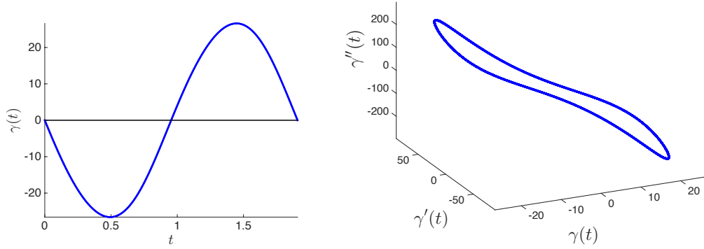
Figure 4: (Left) The periodic solution \gamma(t) . (Right) The first three components of \Gamma(t) , periodic solution of the vector field (83).
