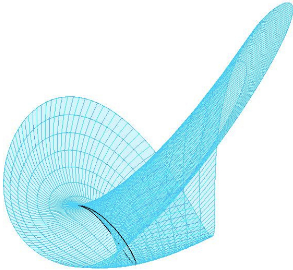
Figure 4: A larger local manifolds for the Arneodo manifold. This Figure illustrates the same manifold shown in Figure 3 however in this case the local approximation is taken to 45 Fourier modes and 40 Taylor modes. We see more nonlinear features of the manifold, but it is more difficult to see the Möbius Strip. Carefully following the boundary curve shows that there is still only one component of the boundary.
