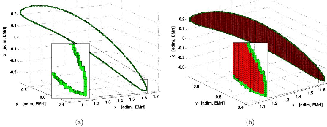
Figure 9: Box covering of the Poincaré map of W_{EM,2}^s
