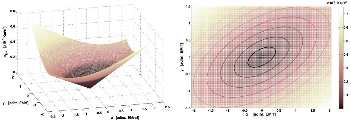
Figure 3: Level curves of \Delta_{EM} for \theta = \pi/3
