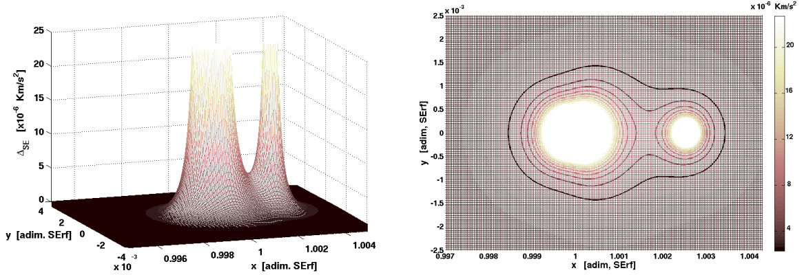
Figure 2: Level curves of \Delta_{SE} for \theta = 0
