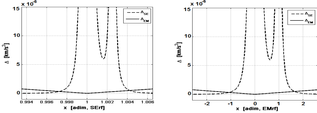
Figure 4: Profile of \Delta_{SE} and \Delta_{EM} , for \theta = 0 , along the Sun-Earth-Moon line. The units of the x -axis are the adimensional Sun-Earth (left) and adimensional Earth-Moon (right).
