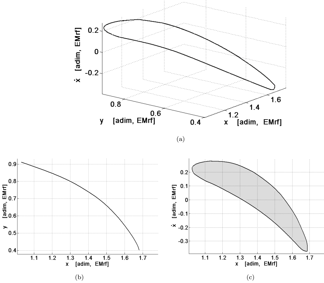
Figure 8: The intersection of W_{EM,2}^s(\gamma_1) with the Poincaré section PS(\theta) is a closed curve in the phase space. (a) Projection of the Poincaré map onto the (x, y, \dot{x}) space. (b) Projection onto the (x, y) plane. (c) In grey the projection of the region \mathcal{B} onto the (x, \dot{x}) plane.
