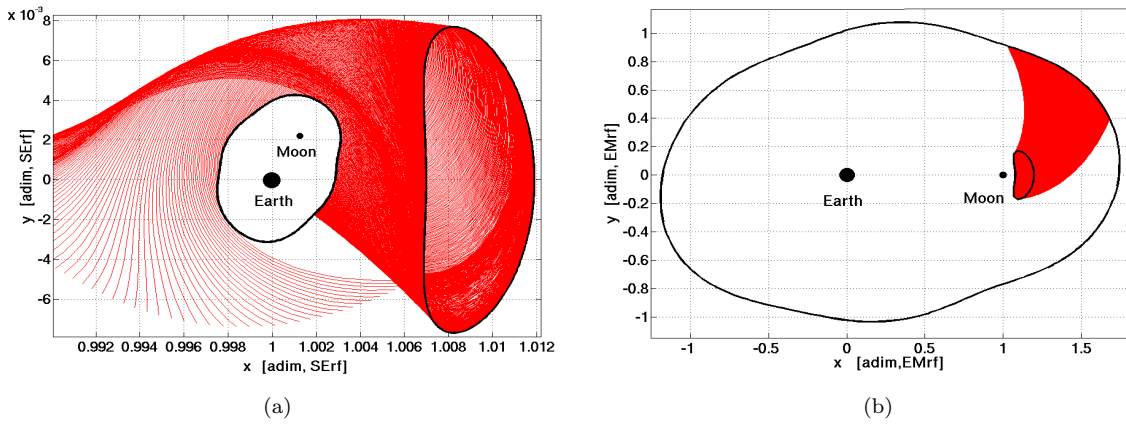
Figure 7: Intersection of W_{SE,2}^u(\gamma_2) and W_{EM,2}^s(\gamma_1) with \Gamma(\pi/3)
