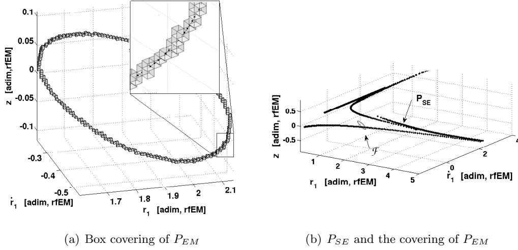
Figure 4: Left: the black dots are the points of P_{EM} covered by the box collection \mathcal{F} . Right: \mathcal{F} and P_{SE} plotted in (r_1, \dot{r}_1, z) cylindrical coordinates.
