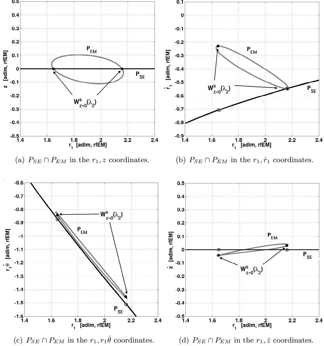
Figure 3: Transfer point definition on suitable Poincaré maps.
