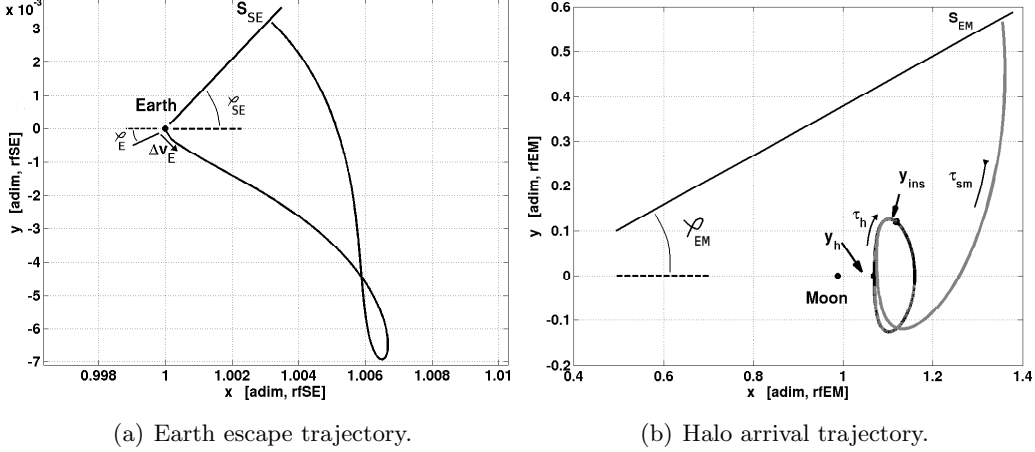
Figure 2: The two stages of the Earth-to-halo trajectory design.
