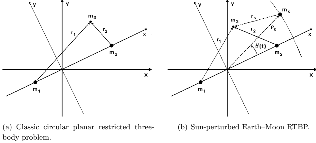
Figure 1: Mathematical models to described the physics of the problem.
