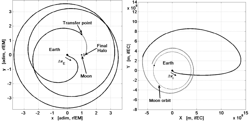
(a) Trajectory in Earth-Moon rotating frame. (b) Trajectory in Earth-centered inertial frame.
