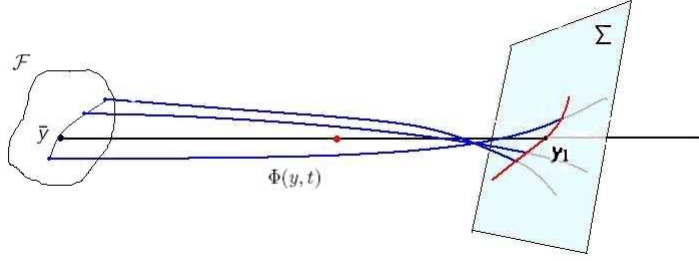
Figure 4: Poincaré section
