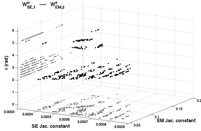
Fig. 7 Zero \Delta V connections between W_{SE,1}^u and W_{EM,2}^s .
