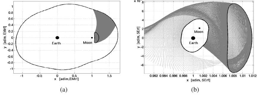
Fig. 5 Intersection of W_{SE,2}^u(\gamma_2) and W_{EM,2}^s(\gamma_1) with \Gamma(\pi/3) .
