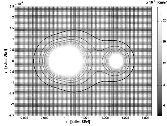
Fig. 2 Level curves of \Delta_{SE} for \theta = 0
