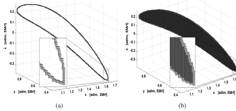
Fig. 6 Box covering of the Poincaré map of W_{EM,2}^S and of the transfer region \mathcal{B} .
