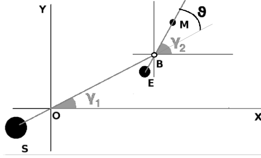
Fig. 1 Positions of the primaries in the inertial reference frame.
