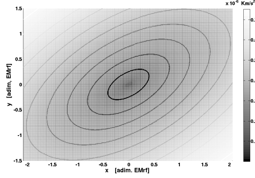
Fig. 3 Level curves of \Delta_{EM} for \theta = \pi/3 .
