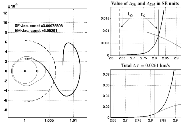
Fig. 9 Example of trajectory. Analysis of the error.
