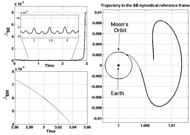
Fig. 8 Example of transfer trajectory and related errors \Delta_{SE} , \Delta_{EM} .
