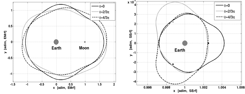
Fig. 4 \Gamma(\theta) with \theta = 0, 2/3\pi, 4/3\pi in EM and SE reference frame.
