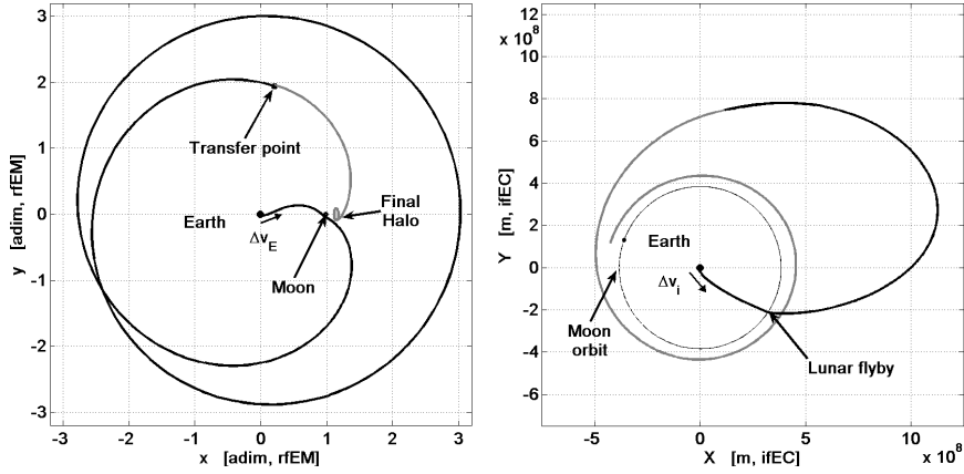
Fig. 5 First guess solution and optimized trajectory corresponding to sol.2 of table 1. (left) First guess solution in Earth–Moon rotating frame. (right) Optimized trajectory in Earth centered inertial frame.
