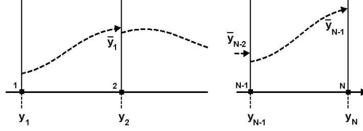
Fig. 4 Direct multiple shooting scheme.
