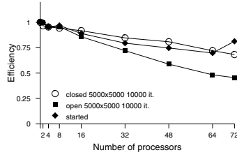
Fig. 2. Parallel execution times in seconds and efficiency for 10000 iterations of our open- and closed-world CA simulators on a 5000 2 matrix. Also, the parallel execution times and efficiency for the last 7500 iterations of our open world simulator.
