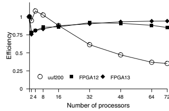
Fig. 3. Parallel execution times in seconds and efficiency for the SAT solver.
