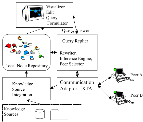
Figure 1: Architecture
