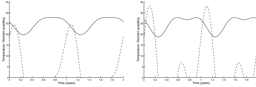
FIGURE 7. Temperature profile and nutrient upwelling for \gamma = 0.5 (left) and \gamma = 1 . In both graphs T_0 = 24.8^\circ C and T_h = 4^\circ C .
