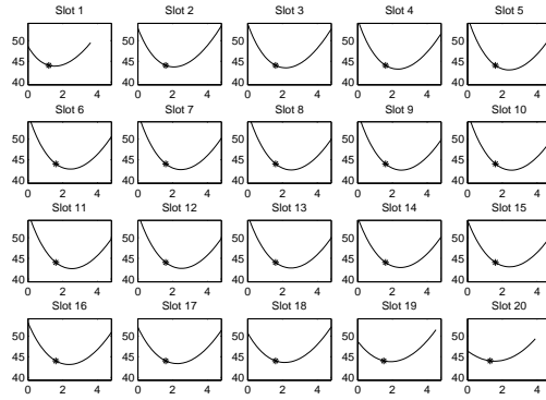
(b) Lag Order III
