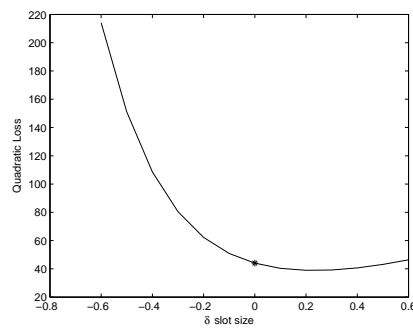
(c) Lag Order III
