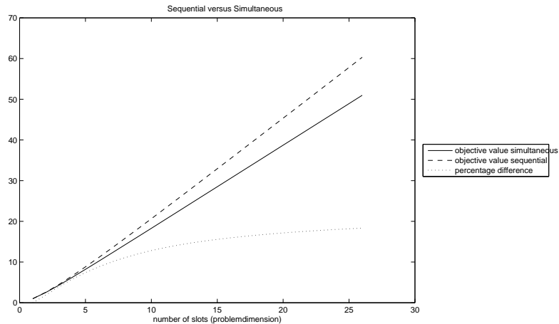
Figure 4.4: The objective values of both optimization approaches and their percentage differences. Quadratic loss, 0 < n < 28 , i.i.d exponential ( \mu=1 ) service times.
