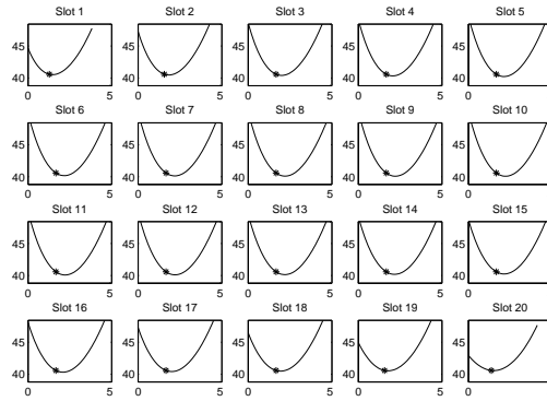
(c) Lag Order IV
