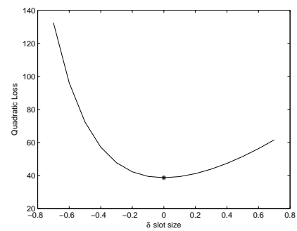
(f) Full Lag Order
