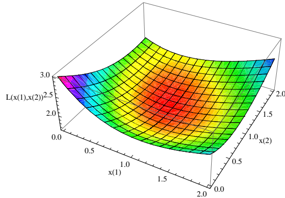
Figure 4.6: Plot of the loss function as a function of x_1 and x_2 . Linear loss, n=3 , i.i.d exponential( \mu=1 ) service times.
