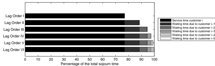
Figure 5.3: Explanation of the lag order terminology.
