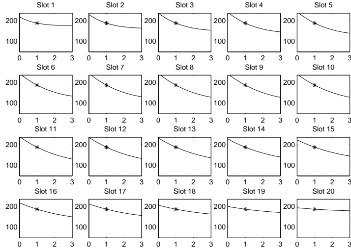
(a) Lag Order I
