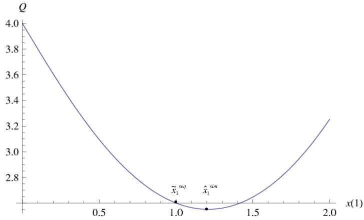
Figure 4.2: Plot of the loss function Q(x_1, 1 + e^{-x_1}) as a function of x_1 . Quadratic loss, n=3 , i.i.d exponential( \mu=1 ) service times.
