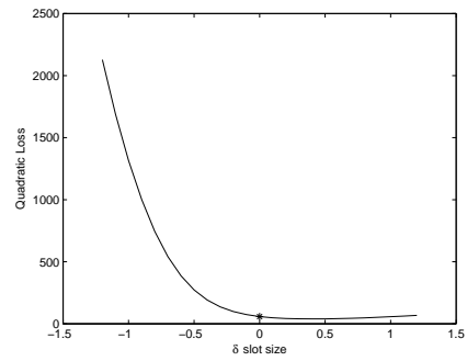
(b) Lag Order II
