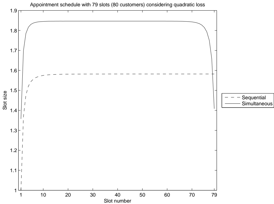
Figure 4.3: The slot sizes of an appointment schedule, optimized using the simultaneous and the sequential approach. Quadratic loss, n=80 , i.i.d. exponential( \mu=1 ) service times.
