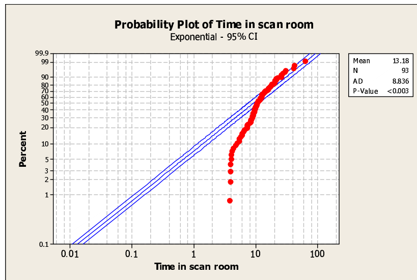
(b) Probability plot for time spend in the CT scan room. As you can see the exponential distribution does not fit the dataset.
