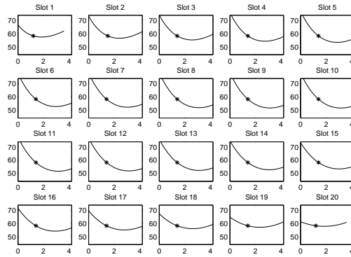
(a) Lag Order II
