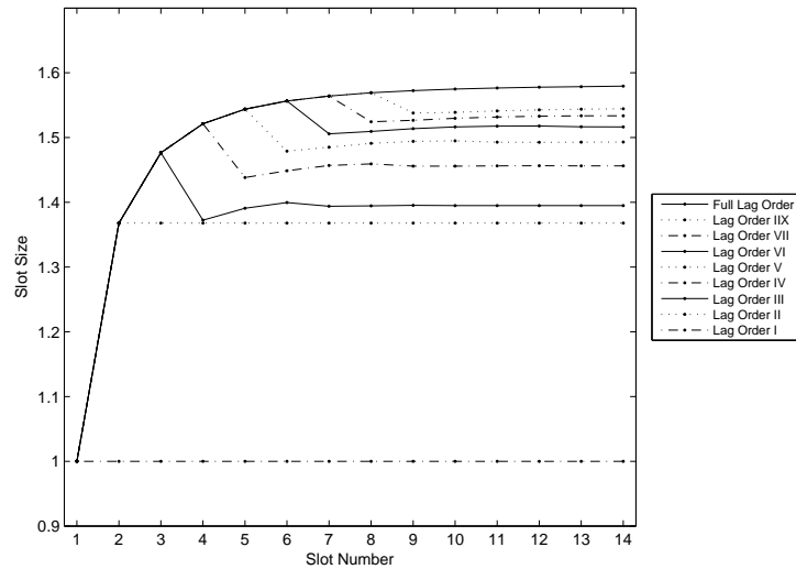
(a) Sequentially optimized schedules for various lag orders. Quadratic loss, n=15 , i.i.d exponential( \mu=1 ) service times.
