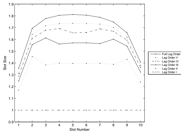
(b) Simultaneously optimized schedules for various lag orders. Quadratic loss, n=11 , i.i.d exponential( \mu=1 ) service times.
