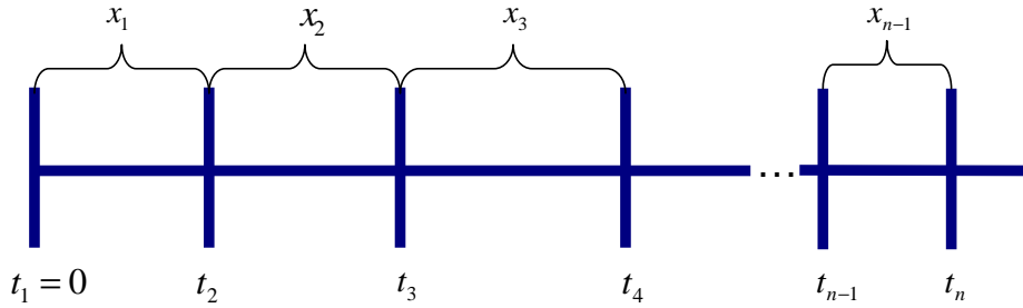
Figure 3.1: The notation used for the time slots and appointment times.
