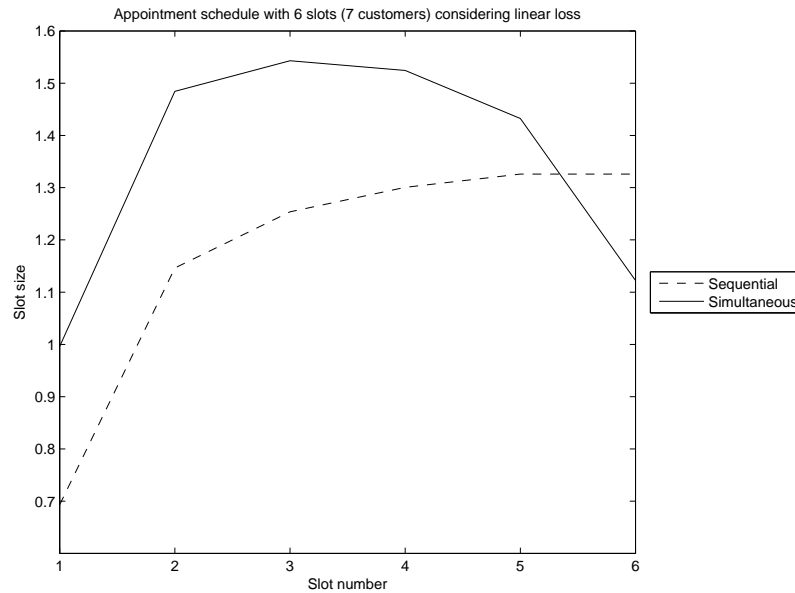
Figure 4.7: Slot sizes of an appointment schedule, optimized using the simultaneous and the sequential approach. Linear loss, n=7 , i.i.d exponential( \mu=1 ) service times.
