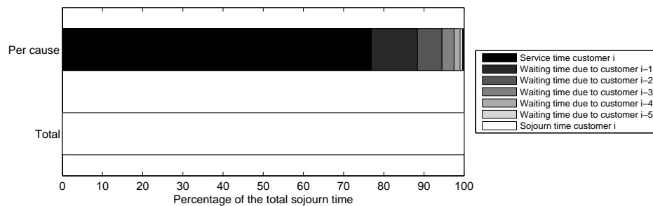
Figure 5.2: Percentage influence on the sojourn time of a customer from the center of an optimized schedule. Service times exponentially ( \mu = 1 ) distributed and we considered the quadratic loss function with n = 30 .
