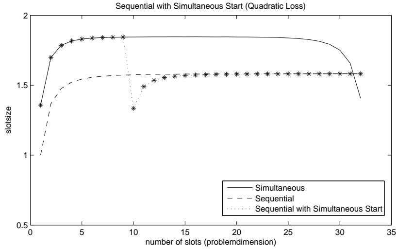
Figure 4.5: First 9 clients according to simultaneous approach continued by sequential approach. Quadratic loss, n=33 , i.i.d exponential( \mu=1 ) service times.
