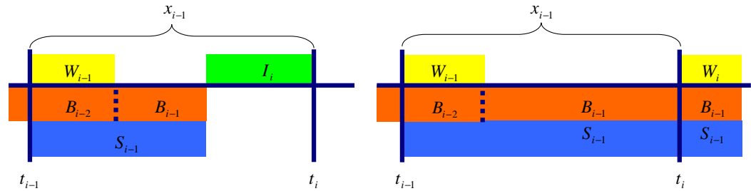
Figure 3.2: Graphical explanation of the relation between the random variables B_i , I_i , W_i and S_i .
