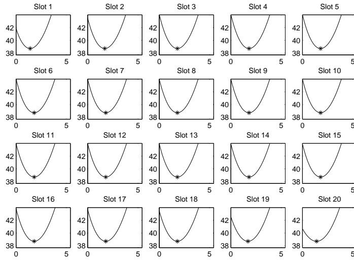
(b) Full Lag Order
