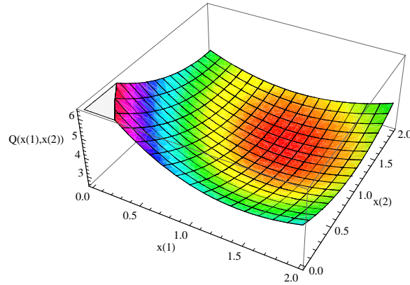
Figure 4.1: Plot of the loss function as a function of x_1 and x_2 . Quadratic loss, n=3 , i.i.d exponential( \mu=1 ) service times.
