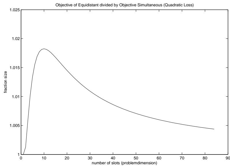
Figure 5.1: The fractional difference in objective of the equidistant approach and the non-equidistant. Quadratic loss, 0 < n < 85 , i.i.d exponential( \mu=1 ) service times.
