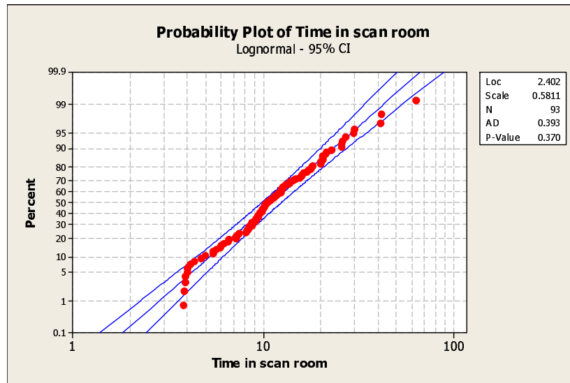
(a) Probability plot for time spend in the CT scan room. We fit the service time with a log-normal distribution.
