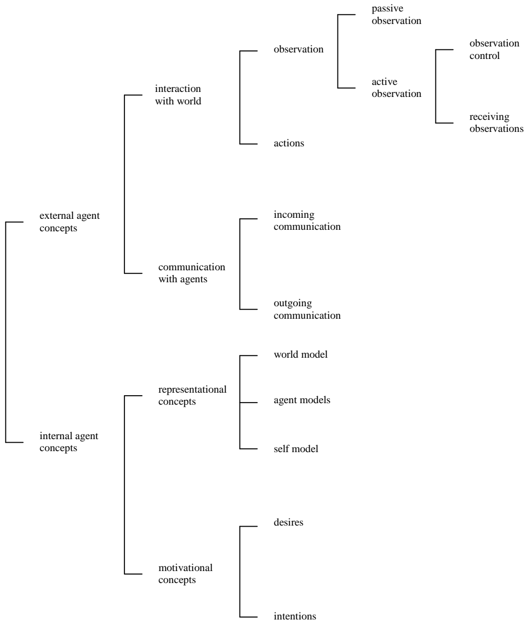
Figure 1 Overview of the types of ontological concepts used
