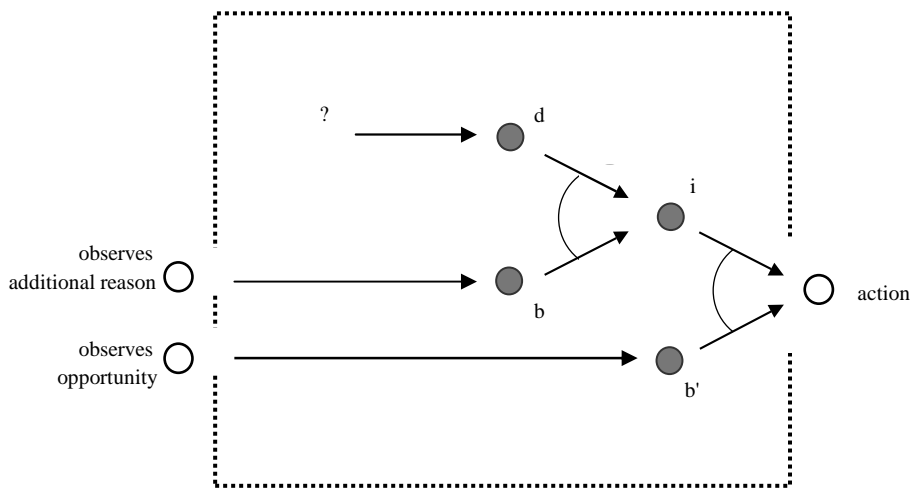
Figure 3 Internal dynamics in a BDI-model for motivation-based behavior
