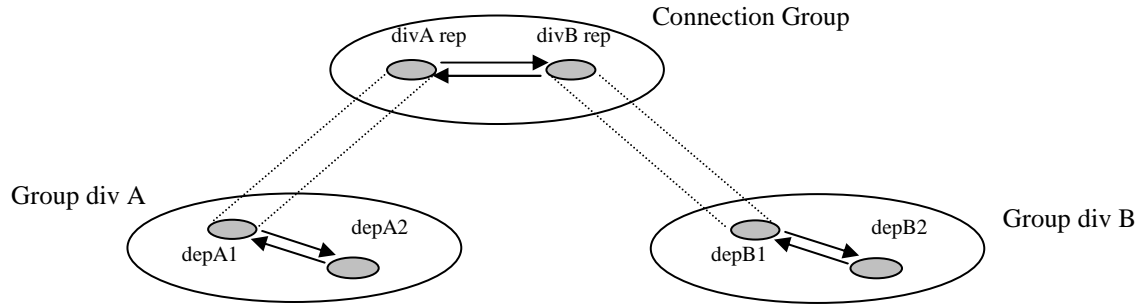
Figure 1. An example AGR organisation structure
