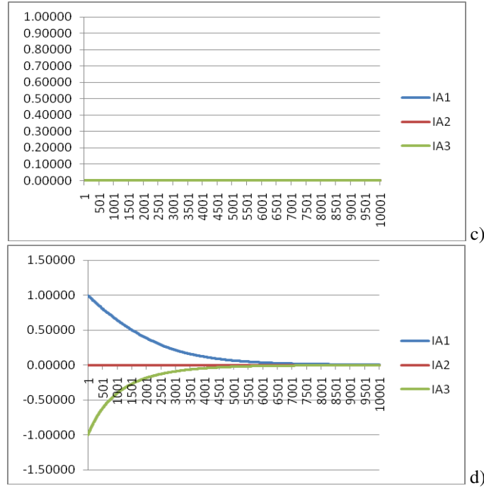
Fig. 4. Dependence on Trust Flexibility: a) \beta = 1 , b) \beta = 0.01 , c) \beta = 0.00 , d) \beta = 0.00 and T_1(0)=1 , T_2(0)=0 , T_3(0)=-1 .
