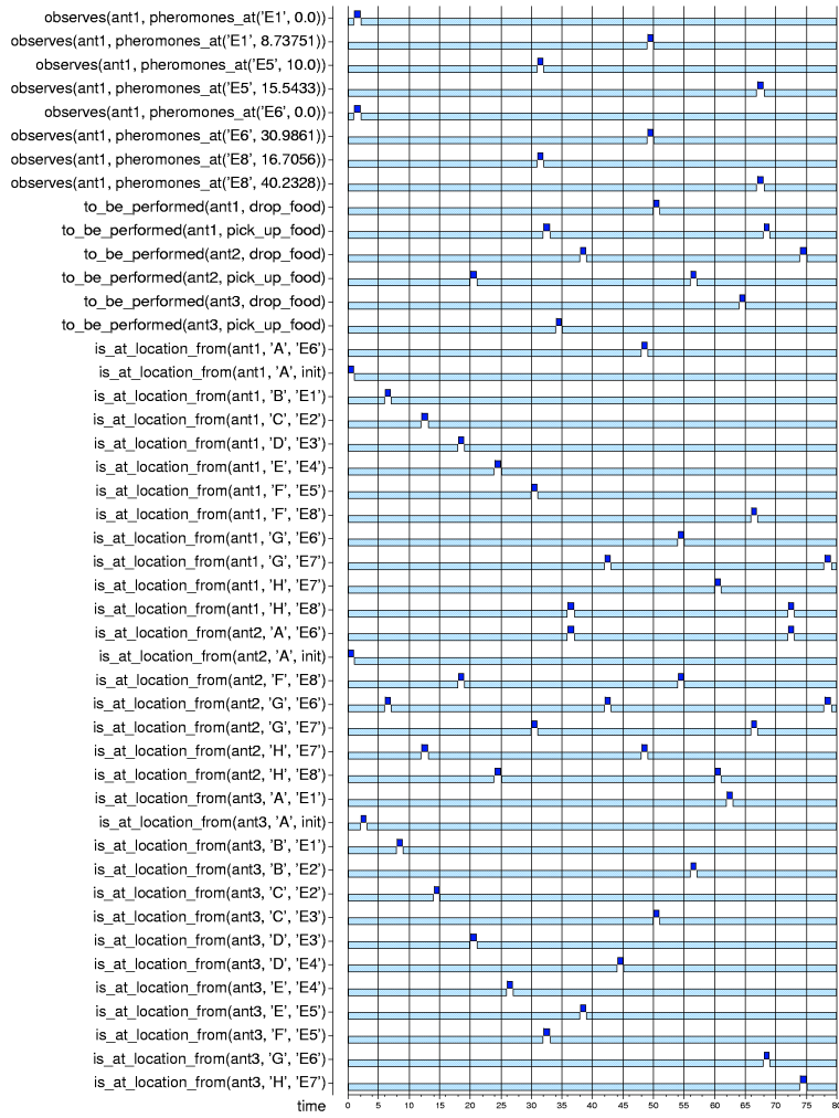
Figure 5: Simulation Trace - Ants Example.
