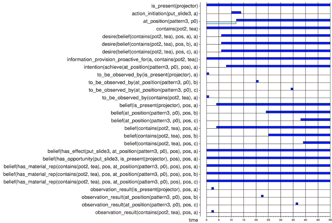
Figure 6: Simulation Trace - Slide Example.
