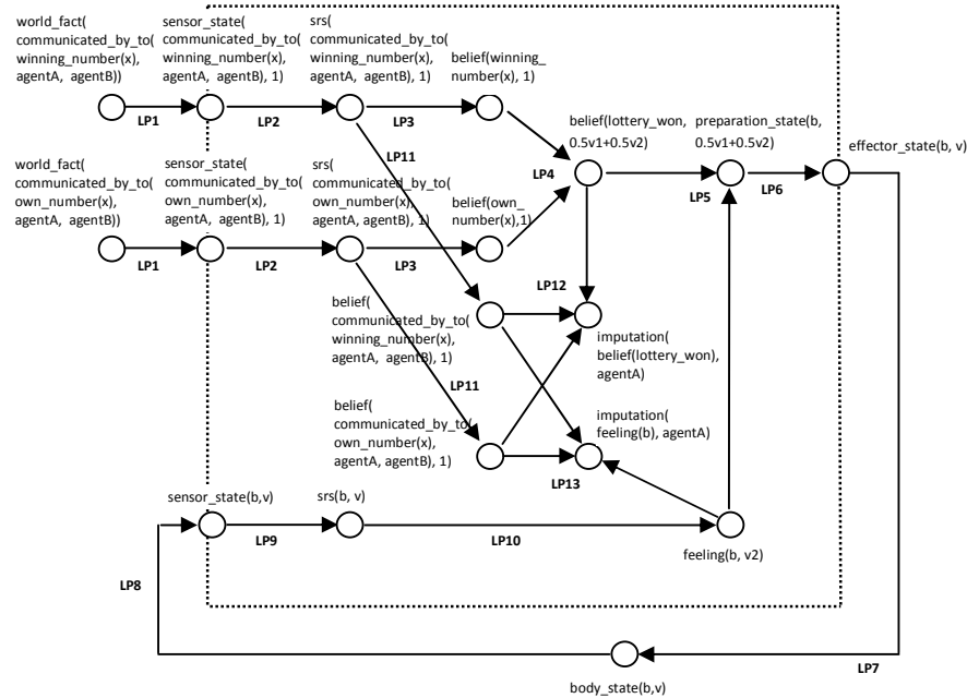
Figure 3: Overview of the agent model for the observing agent B
