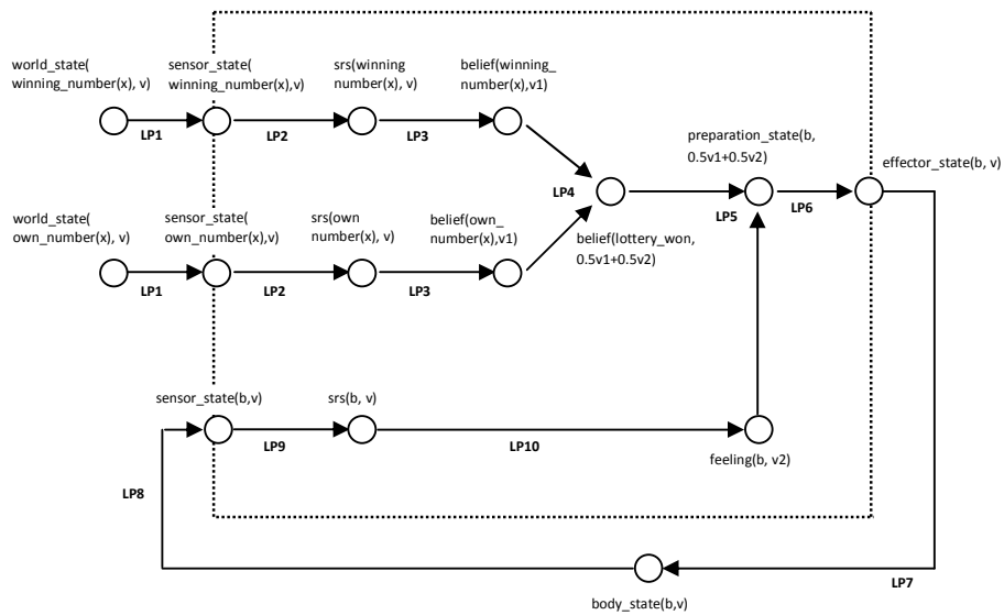
Figure 2: Overview of the agent model for the observed agent A
