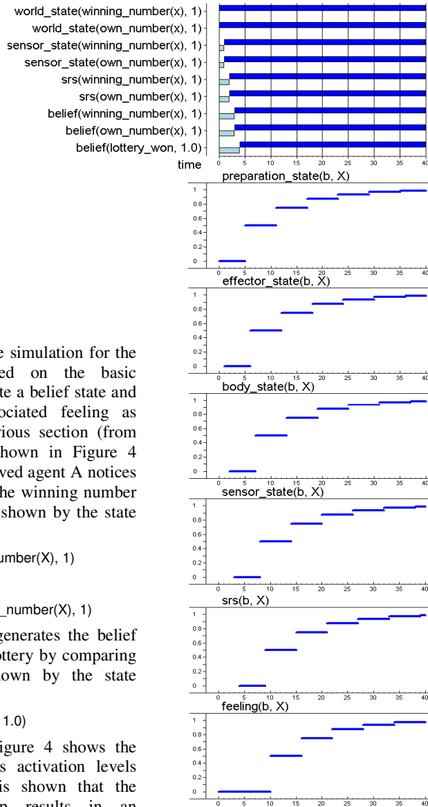
Figure 4: Example simulation trace for the observed agent
