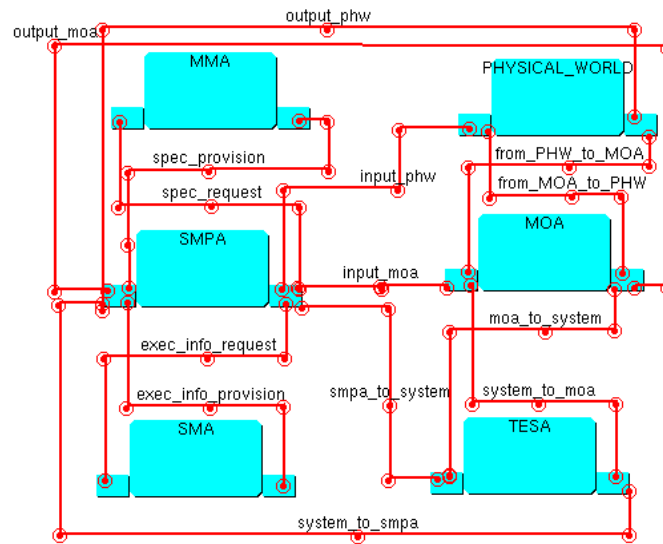
Fig. 1. Overview of the multi-agent system architecture.
