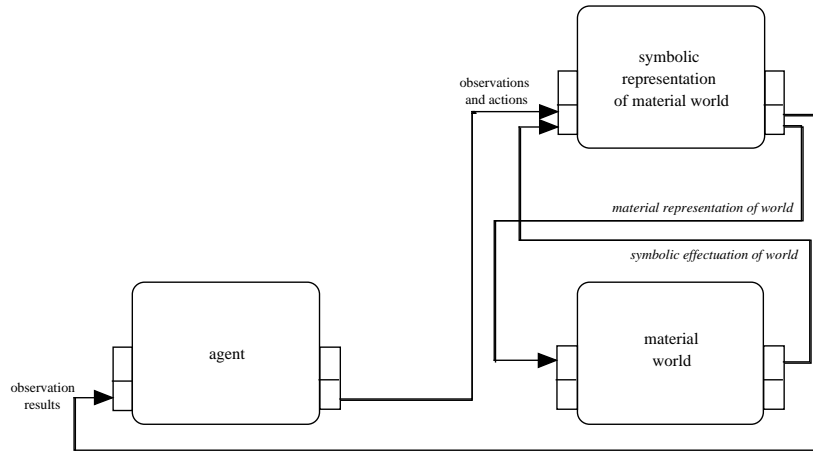
Fig. 7. Transduction and symbolic links connecting agent and material world
