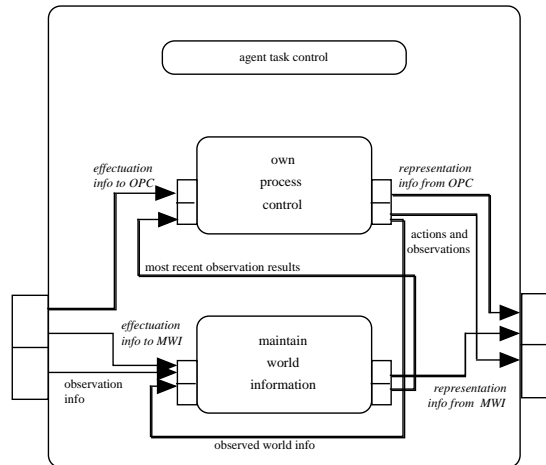
Fig. 11. Links within the agent
