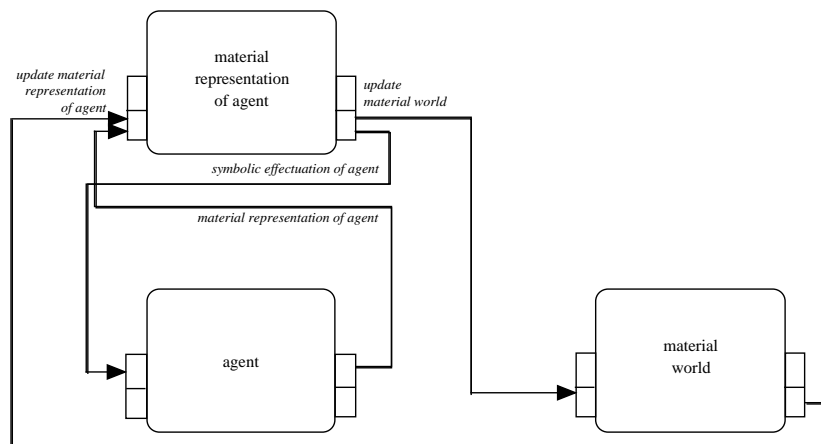
Fig. 9. Transduction and material links connecting material world and agent
