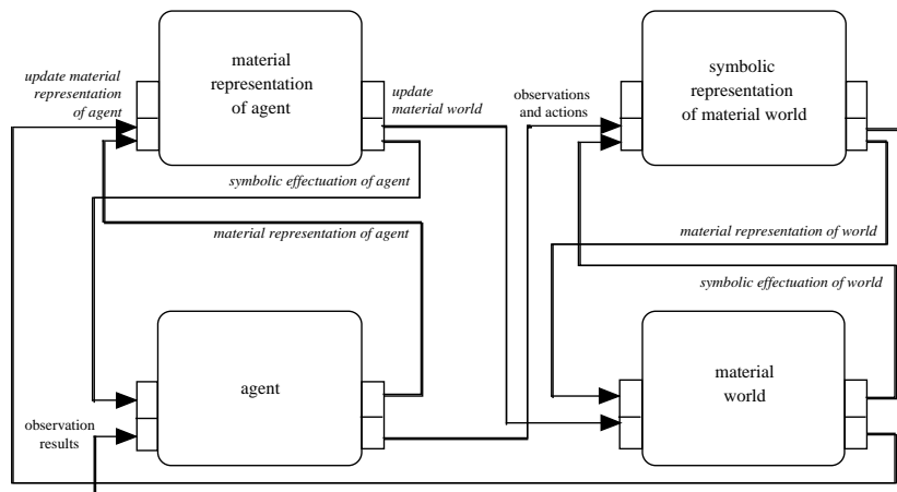
Fig. 10. Transduction, symbolic and material links connecting agent and material world
