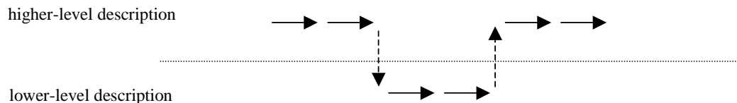
Fig. 3 An interacting trace as a basis for a composite explanation
