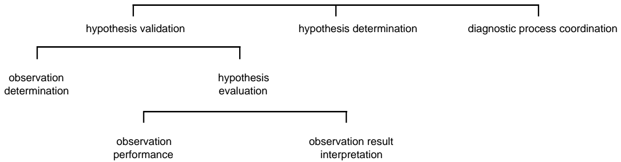
Figure 2. Tasks within a task model for diagnostic reasoning based on anti-causal knowledge.
