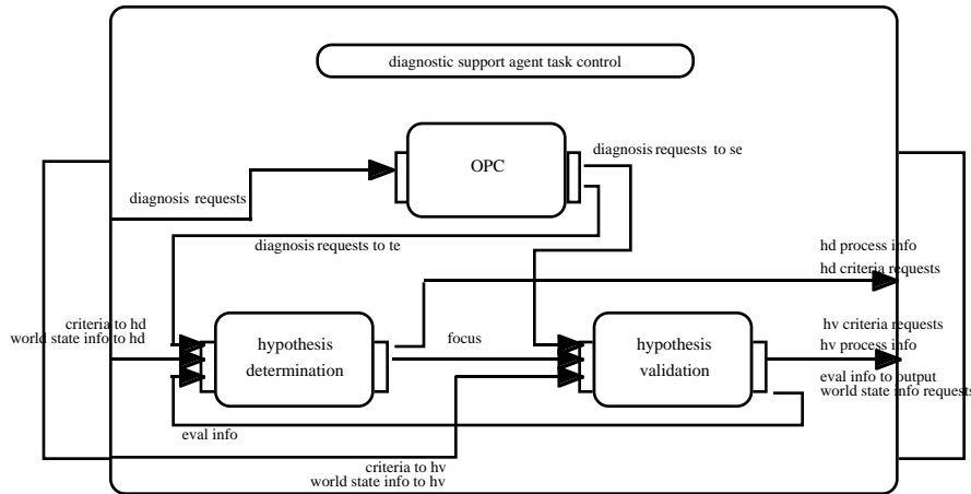
Figure 14. Top level composition of the diagnostic support agent.
