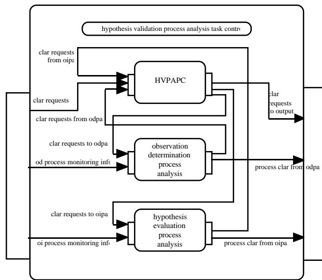
Figure 20. Composition of hypothesis validation process analysis.
