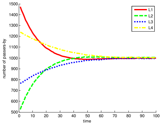
Figure 4. Agent-based model - simulation results with complex function
