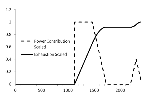
Figure 15. The participant's estimated power contribution and the exhaustion build-up in time.
