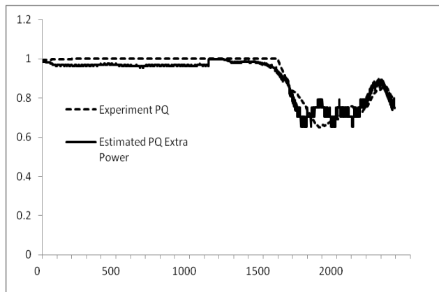
Figure 15. PQ of participant 2 in 1 block and the fitted estimated PQ curve.
