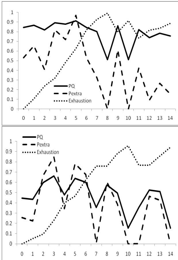
Figure 7 Performance, power and exhaustion for task demands of 15 and 25; logistic case B.
