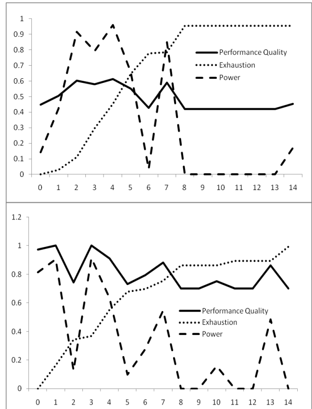
Figure 4: Performance, Power and Exhaustion for task demands of 15 and 25 without allowing for recovery.
