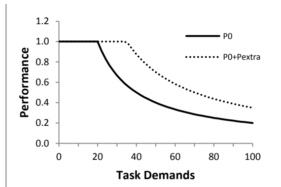
Figure 2 Proportional degradation curve
