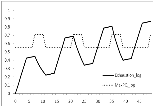
Figure 10 Exhaustion and Performance Quality in the situation with varying Task Demands.
