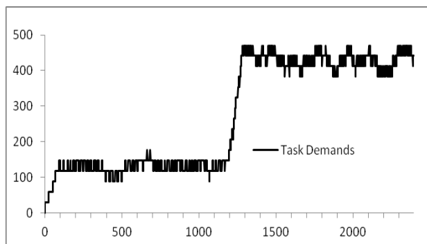
Figure 12. Task Demands from 1 experimental block.
