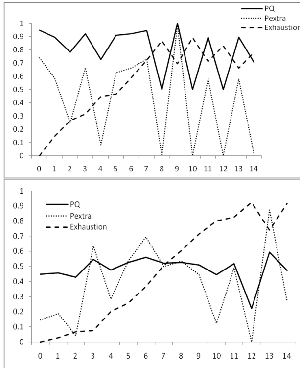
Figure 5. Performance, power and exhaustion for task demands of 15 and 25, proportional case
