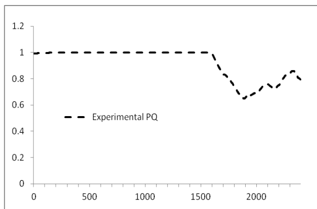
Figure 13. Performance Quality of participant 2 during 1 block.
