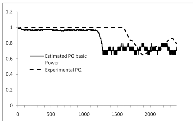
Figure 14. PQ of participant 2 during 1 block and the estimated PQ with basic effort contribution.
