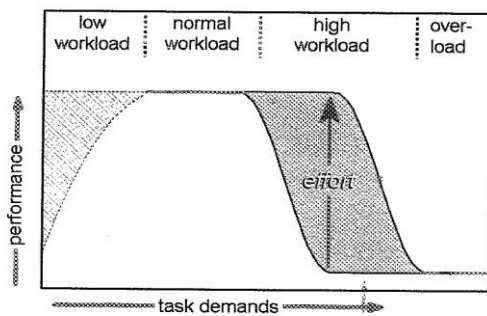
Figure 1 Hypothetical relation between task demands, effort and performance. Adapted from [7]
