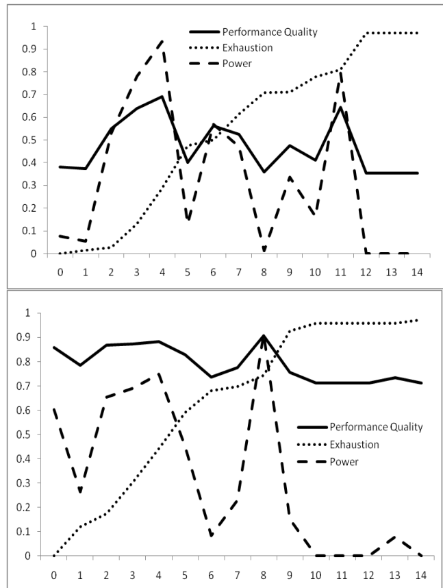
Figure 6. Performance, power and exhaustion for task demands of 15 and 25 without allowing for recovery; logistic case A.
