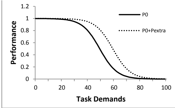
Figure 3 Logistic degradation curve
