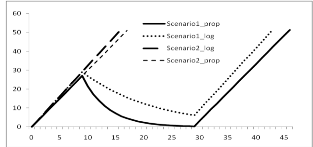
Figure 8 Exhaustion for scenario 1 and 2.
