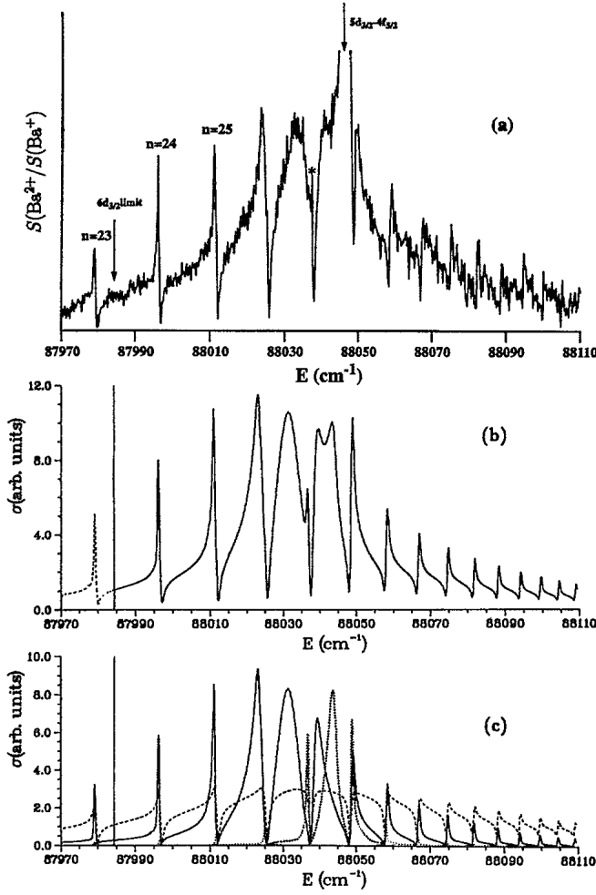
FIG. 3. Excitation spectra of 4f_{5/2}7h J' levels from the metastable 5d^2\ ^1G_4 level via the 5d_{3/2}7h[11/2] J=5 level, followed by photoionization of \text{Ba}^+ 6d_{3/2} and 7s ions. The energy scale is relative to the 6s^2\ ^1S_0 ground state. (a) Experimental spectrum; the \text{Ba}^{2+} signal is divided by the \text{Ba}^+ signal to account for instabilities in the production of metastables and laser power fluctuations. The narrow resonances were identified as 6d_{5/2}ni levels. The 6d_{5/2}27i J'=4 at 88\,037\text{ cm}^{-1} is denoted by (*). (b) Theoretical spectrum calculated with the eigenchannel R -matrix method. (c) The relative contributions of each final J' value to the theoretical spectrum in (b); dotted line, J'=4 ; full line, J'=5 ; dashed line J'=6 .
