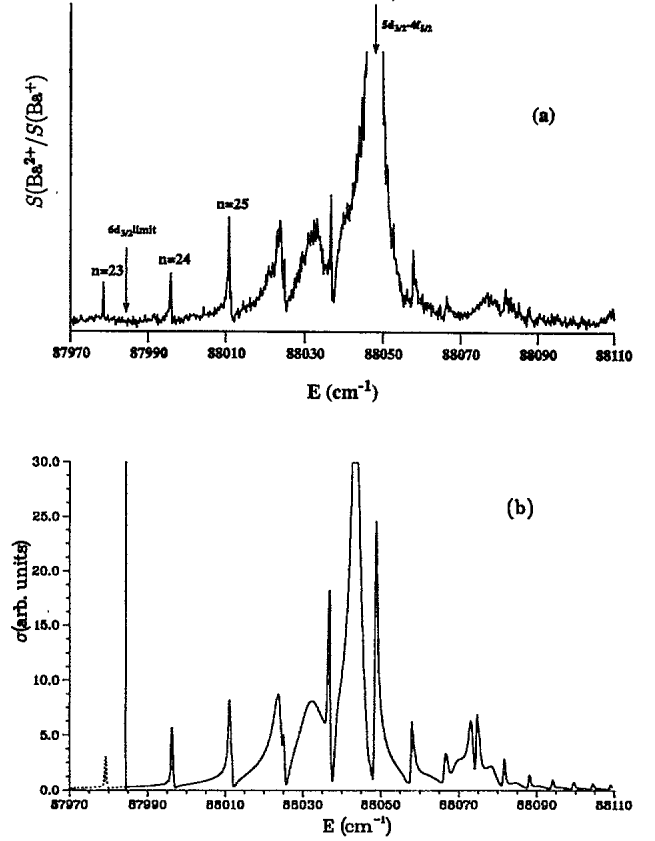
FIG. 4. (a) Experimental spectrum of the excitation of 4f_{5/2}7h J' levels from the metastable 5d^2\ ^3F_4 level via the 5d_{3/2}7h[9/2] J=5 level, followed by photoionization of \text{Ba}^+ 6d_{3/2} and 7s ions. (b) Theoretical spectrum calculated with the eigenchannel R -matrix method. The energy scale is relative to the 6s^2\ ^1S_0 ground state.
