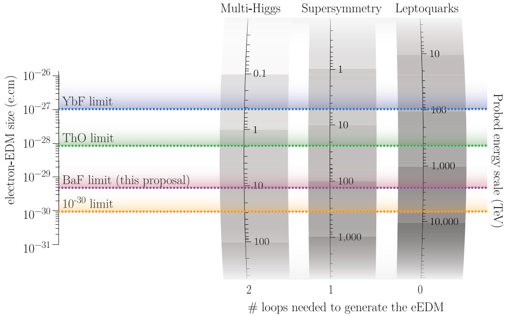
Fig. 1. The experimental upper limits, on the value of e\text{EDM} , translated into a limit on the probed energy scale through d_e = e\alpha^n \sin \phi (m_e/\Lambda^2) . Here \alpha is the fine-structure constant and n is the number of loops needed to generate the e\text{EDM} . \phi is a typical CP -violating phase, which is set to the maximum value of \pi/2 , and \Lambda is the energy scale that is being probed. The regions above the dotted lines are the energy ranges that are excluded for the indicated classes of models. The models differ in the number of loops required to generate an e\text{EDM} . The e\text{EDM} value predicted by the SM, in which the e\text{EDM} only appears at four-loop level, is of the order of 10^{-38} e.cm.
