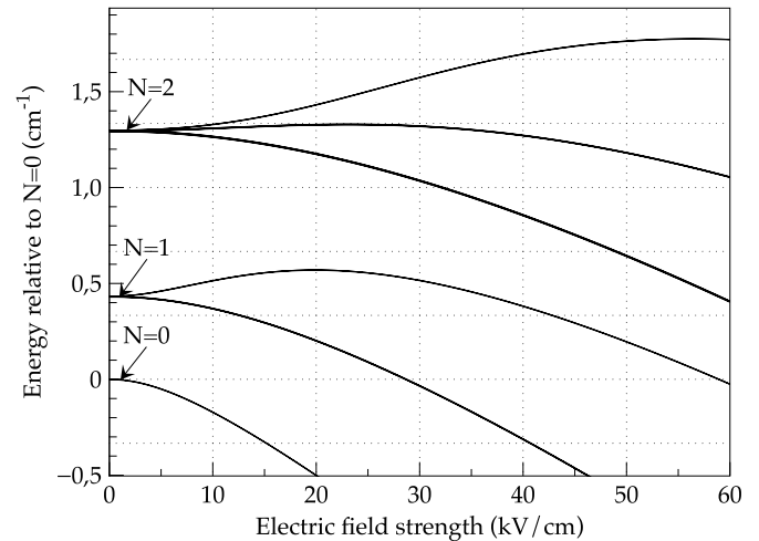
Fig. 6. The lowest three rotational levels within the electronic ground state of the BaF molecule, as a function of electric field strength. The N = 0 level is used for the e EDM measurement; deceleration is most efficient in the N = 2 level, while lasercooling and detection is best performed in the N = 1 level.
