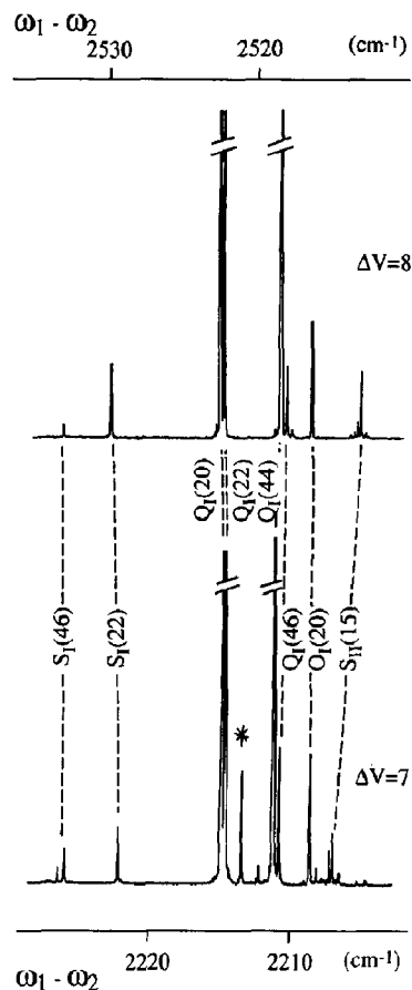
Fig. 2. Corresponding Raman resonances of adjacent overtones in the \Delta\nu=7 (lower spectrum) and \Delta\nu=8 (upper spectrum) CARS spectra. The line denoted by the asterisk is the S_{II}(58) .
