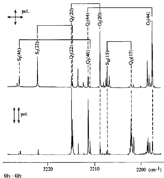
Fig. 3. Polarization effects in the \Delta v=7 resonance-enhanced CARS spectrum. Upper spectrum: crossed polarizations of beams with frequencies \omega_1 and \omega_2 . Lower spectrum: parallel polarizations. Both polarizations are linear.
