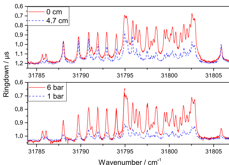
Fig. 3. The Q-branch region of the 0–0 band of the C–X transition at different experimental conditions. Top panel compares a CRDS measurement close to the nozzle orifice (red) and 4.7 cm down (blue). The bottom panel compares a high backing pressure of C 2 H 2 /Ar of 6 bar (red) with a lower pressure of 1 bar (blue). (For interpretation of the references to colour in this figure legend, the reader is referred to the web version of this article.)
