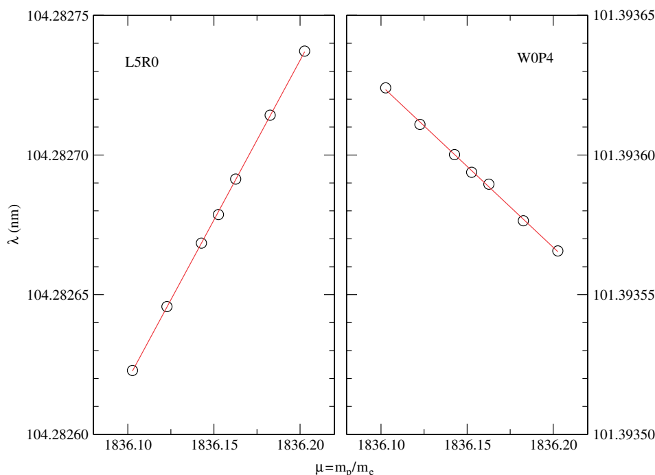
Figure 4. The wavelengths of the B^1\Sigma_u^+(v=5) \leftarrow X^1\Sigma_g^+(v=0) R(0) and C^1\Pi_u(v=0) \leftarrow X^1\Sigma_g^+(v=0) P(4) transitions were deduced using calculations based on ab initio adiabatic potentials for seven different values of the proton-to-electron mass ratio around the presently known value. The sensitivity coefficients K_i are deduced from the slope of the linear regression of these points.
