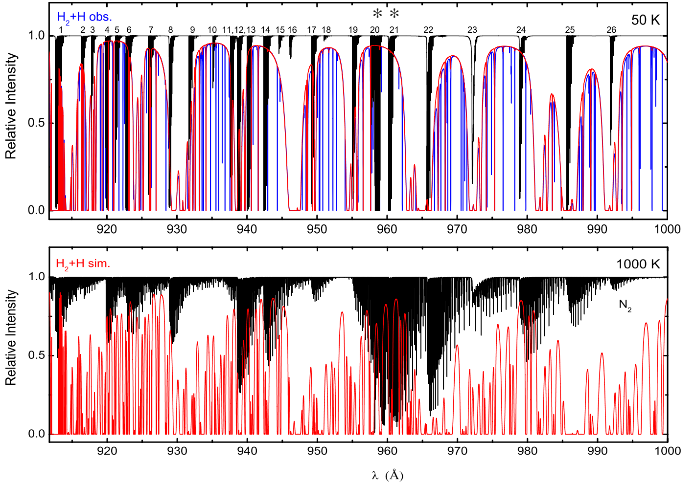
Fig. 4. Simulated absorption spectra for N 2 (black) and H 2 +H (red) in the wavelength range 912–1000 Å assuming thermal excitation temperatures of 50 K ( top ) and 1000 K ( bottom ). The column density of N 2 is 10 15 cm -2 and values for H 2 and H are taken to be half of the observed column densities in the well-studied diffuse cloud toward ζ Oph, as is appropriate for the center of the cloud: N(\text{H}_2) = 2.1 \times 10^{20} and N(\text{H}) = 2.6 \times 10^{20} cm -2 . The model H 2 Doppler width is 3 km s -1 . Also shown is the H 2 + H absorption spectrum (blue) toward ζ Oph using the observed column densities for individual J levels, showing enhanced non-thermal excitation of H 2 in the higher J levels. The asterisks indicate the c'(0) (Band 20) and c(0) (Band 21) bands, respectively, detected in absorption toward HD 124314.
