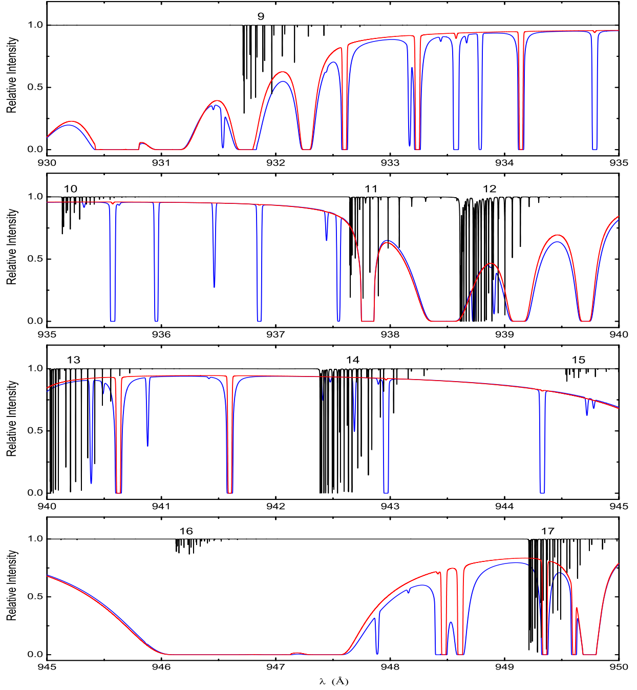
Fig. B.2. As Fig. B.1, but for 930–950 \text{\AA} .
