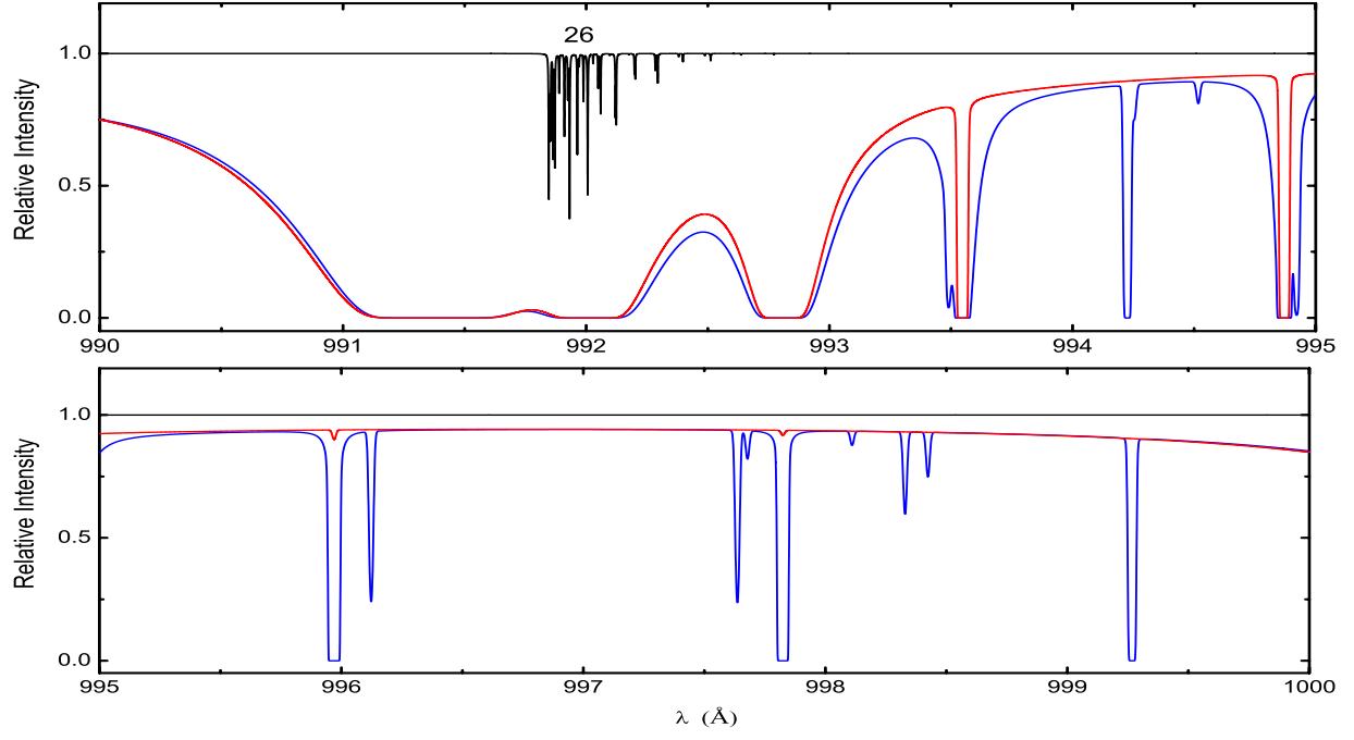
Fig. B.5. As Fig. B.1, but for 990–1000 \text{\AA} .
