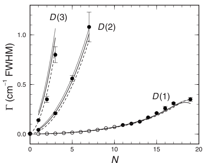
FIG. 10. Vibrational and rotational dependence of predissociation level widths for the 3p\sigma_u D^3\Sigma_u^+ Rydberg state of ^{14}\text{N}_2 . Full circles: Present fine-structure-averaged experimental widths. Open circles: F_1 widths of Ref. 6. Curves: Present CSE-model results (Solid: F_2 , dashed: F_1 , and dotted: F_3 ). The turning over of the D(v=1) model widths in the region of N=19 is caused by the crossing of D(v=1) in this region by the higher-lying valence level C^3\Pi_u(v=13) which has a lower rotational constant.
