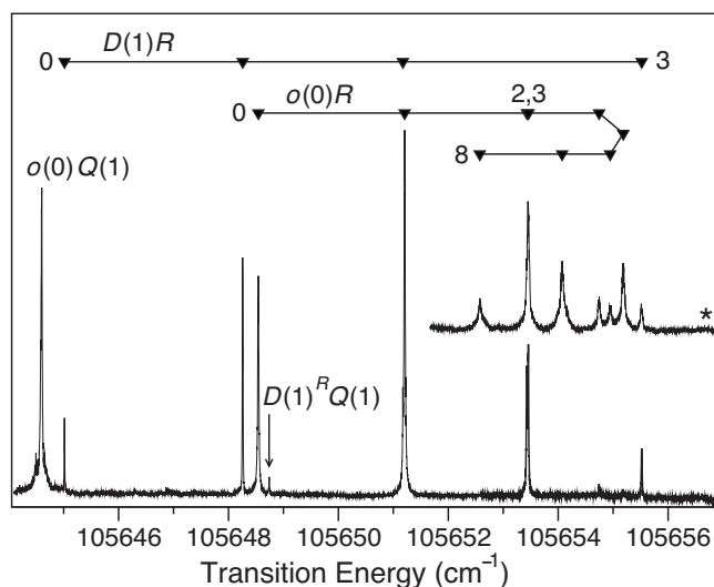
FIG. 3. 1 XUV+1 UV ionization spectrum of the R branches of the o\ ^1\Pi_u-X\ ^1\Sigma_g^+(0,0) and D\ ^3\Sigma_u^+-X\ ^1\Sigma_g^+(1,0) bands in ^{15}N_2 , recorded using the PDA-based XUV source. Nozzle-skimmer distance=150 mm, except for the scan labeled with an asterisk where the nozzle-skimmer distance = 0 mm.
