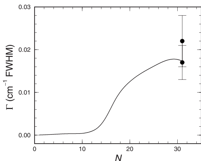
FIG. 11. Rotational dependence of predissociation width for the D(v=0) level of ^{14}N_2 . Solid curve: Computed CSE-model widths for the F_2 sublevel. Solid circles: Experimental linewidths from NIR spectrum for P_i(32) lines from D-E(0,0) band (see text).
