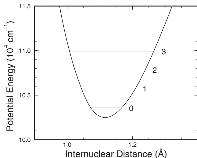
FIG. 8. Model diabatic potential-energy curve for the D\ ^3\Sigma_u^+ state of N_2 , relative to the v=0, J=0 level of the X\ ^1\Sigma_g^+ state. Observed energies for the D(v=0-3) levels of ^{14}N_2 are also shown.
