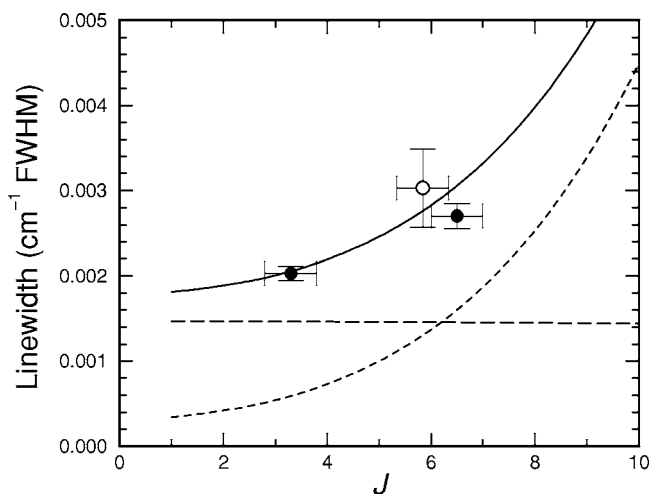
FIG. 2. Comparison between experimental (circles) and CSE (curves) rotational dependences of linewidths for the b\ ^1\Pi_u(v=1) level of ^{14}\text{N}_2 . Solid circles: widths from experimental lifetimes of Ref. 4 and this work, open circle: width from experimental lifetime of Ref. 1, long-dashed curve: radiative width, dashed curve: predissociative width, and solid curve: total width.
