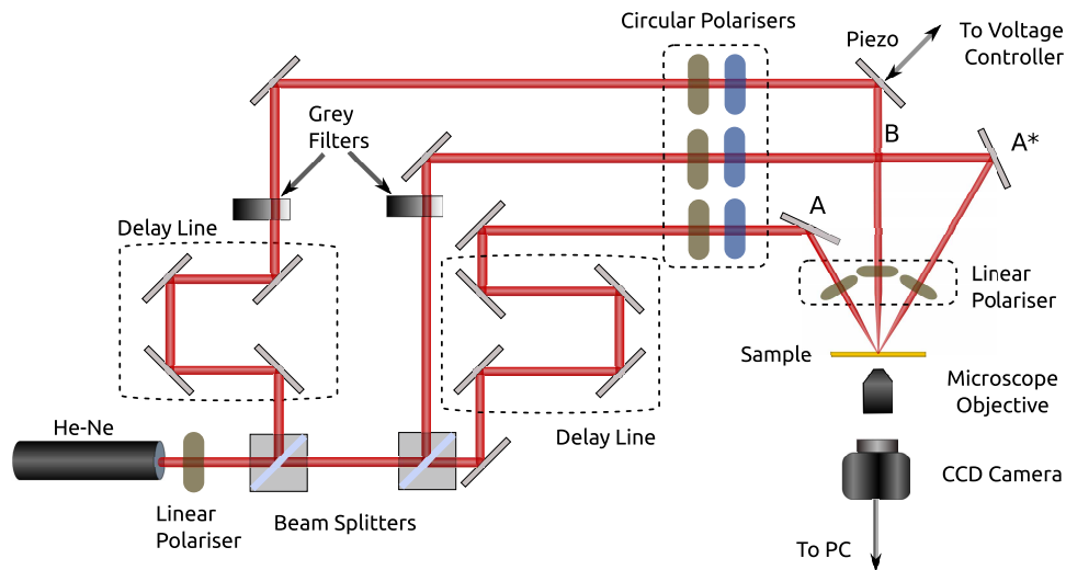
Fig. 3. Sketch of the experimental setup. The sample is illuminated from the glass-substrate side.
