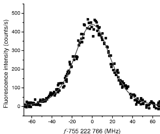
Fig. 2. An example of the measured fluorescence spectrum for the 4s^2S_{1/2} - 4p^2P_{1/2} transition in \text{Ca}^+ and the corresponding Voigt fit
