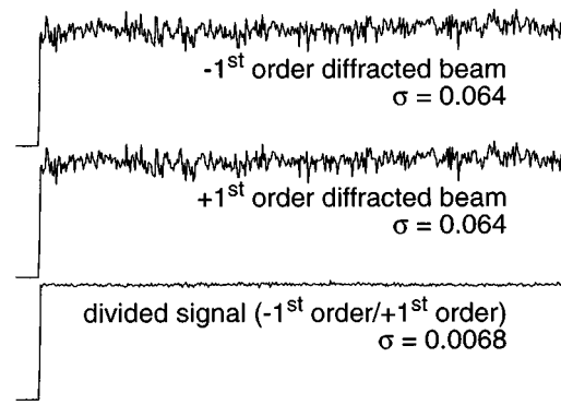
Fig. 2. Measured XUV intensity at -1st (upper trace) and +1st (middle trace) -order diffracted beams. The noise in both cases is approximately 6% for a 1-s (10 laser pulses) averaging time. The lower trace shows a ratio spectrum, with a noise reduction by one order of magnitude to 0.68% rms. The horizontal scale represents a time series.
