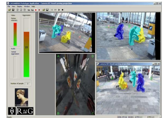
Action Recognition
