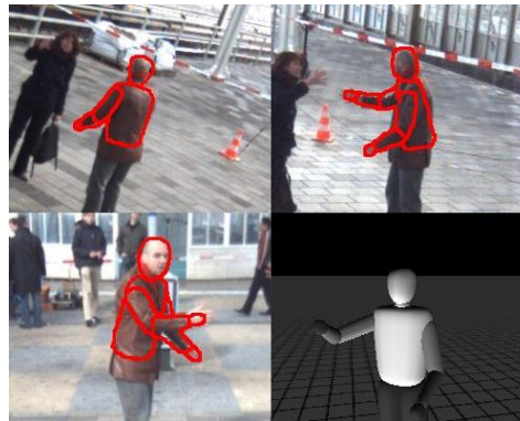
Pose Recovery
