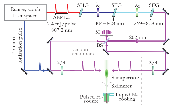
FIG. 2. Schematic overview of the experimental setup. Amplified comb pulse pairs are frequency up-converted in sequential doubling (SHG) and mixing (SFG) stages in \beta -barium borate. Between each stage, a special wave plate ( \lambda_1 and \lambda_2 ) rotates the polarization to maintain type-I phase matching. The generated 201.80 nm beam is split equally by a metallic beam splitter (BS) where they recombine again after one round-trip to form a Sagnac interferometer (SI). The molecular beam is formed from a pulsed supersonic expansion and is collimated by a skimmer and subsequent slit aperture.
