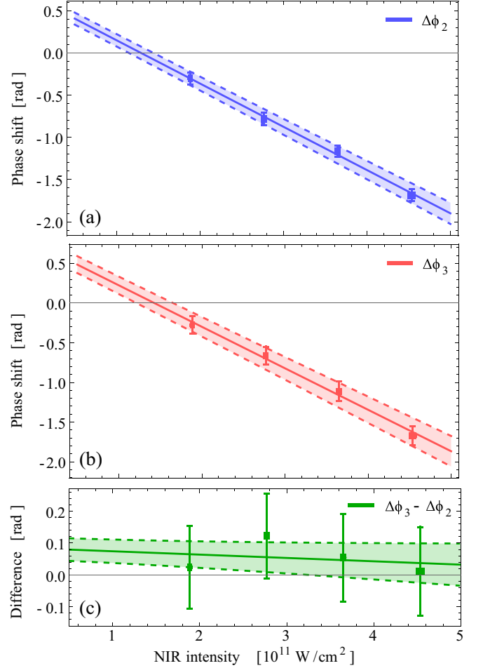
FIG. 11. The observed phase shift of the Ramsey fringe in the VUV as a function of NIR intensity in the interaction region for (a) \Delta N = 2 , (b) \Delta N = 3 , and (c) their difference. The solid line represents a linear fit of the data and the shaded area indicates the 1\sigma uncertainty interval. A maximum shift of 1.65 rad was observed by increasing the intensity in the interaction region by a factor of 4.6. However, the fitted slopes of the curves at \Delta N = 2 and \Delta N = 3 are almost equal, with a small residual difference between \Delta N = 2 and \Delta N = 3 , as is shown in panel (c), due to drifts of the setup as the measurements were performed sequentially (see text).
