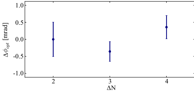
FIG. 12. The relative optical phase shift of the fundamental beam at 770 nm as a function of the pulse delay (equal to \Delta NT_{\text{rep}} ). The data points are obtained by averaging over 15 measurements, each with a statistical uncertainty of 1.5–2.5 mrad. This is equivalent to a typical measurement day. The average differential phase stability is considerably better than 1 mrad.
