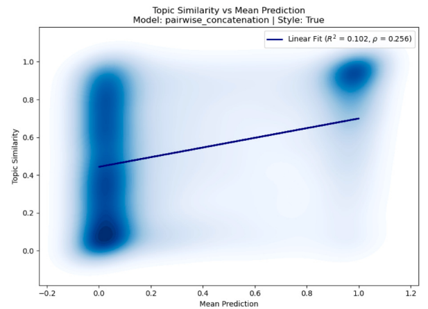
Fig. C.12. Pairwise concatenation model with style features (LDA-based topic similarity). Slightly increased topic correlation.
