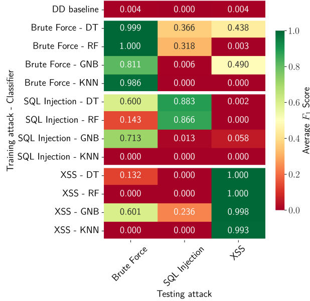
Figure 4.3: Classifier performance in detecting known and novel web attacks on the CIC-IDS-2018 dataset
