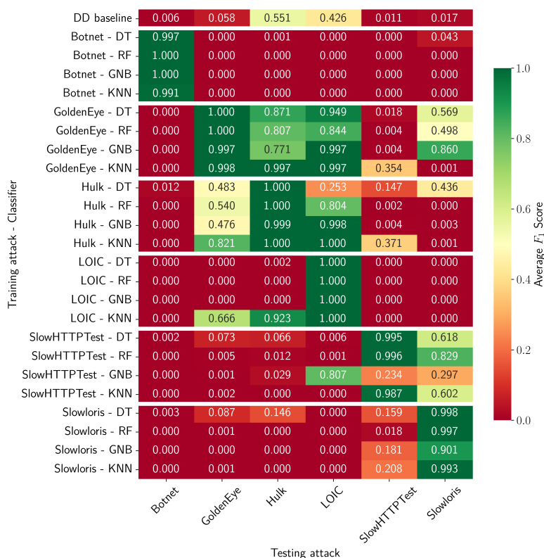
Figure 4.4: Classifier performance in detecting known and novel (D)DoS attacks on the CIC-IDS-2017 dataset
