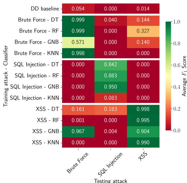
Figure 4.2: Classifier performance in detecting known and novel web attacks on the CIC-IDS-2017 dataset
