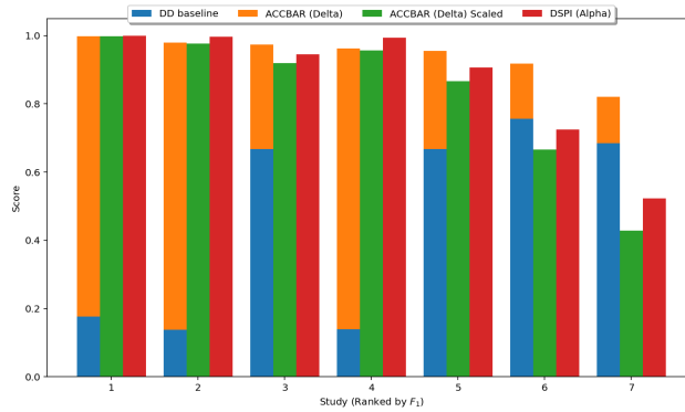
Figure 5.3: Performance indicator scores of DSPI and ACCBAR on the F_1 score for seven studies
