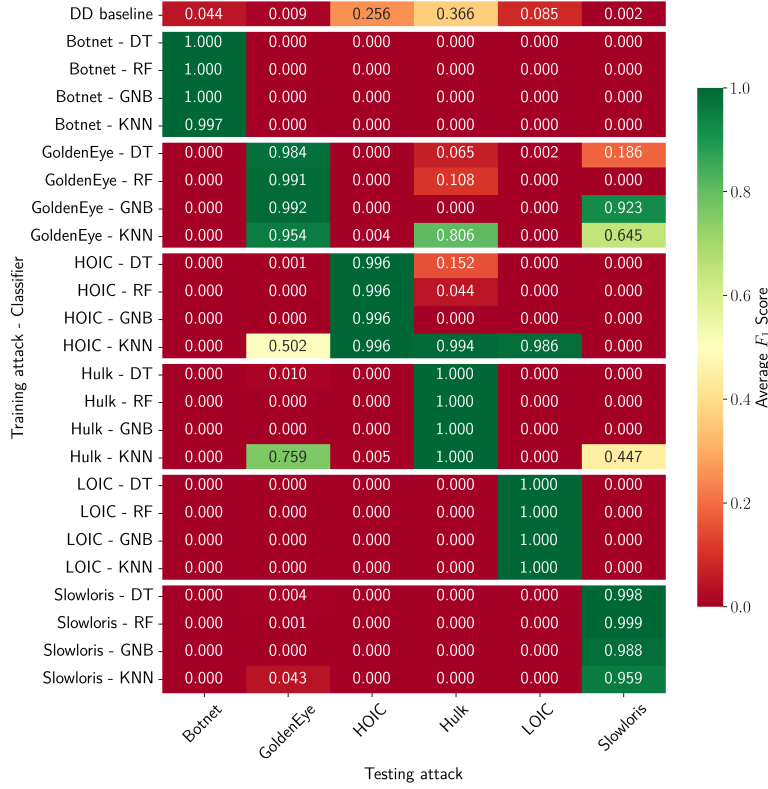
Figure 4.5: Classifier performance in detecting known and novel (D)DoS attacks on the CIC-IDS-2018 dataset
