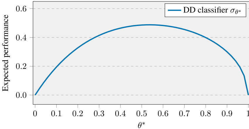
Figure 3.1: Expected DD classifier performance for G-mean 2 with M = 50 and P = 5
