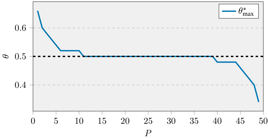
Figure 2.2: Example of non-trivial \theta_{\max}^* for G_{\theta}^{(2)} with M = 50
