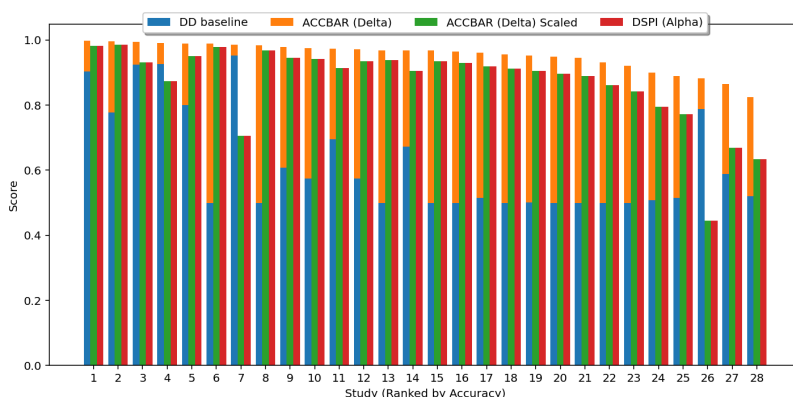
Figure 5.2: Performance indicator scores of DSPI and ACCBAR on accuracy for 28 different studies
