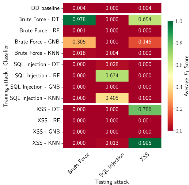
Figure 4.6: Classifier performance trained on CIC-IDS-2017 web attacks to detect CIC-IDS-2018 web attacks
