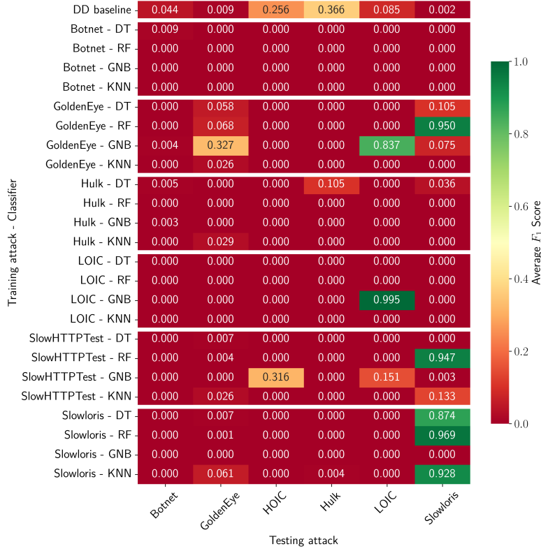
Figure 4.7: Classifier performance trained on CIC-IDS-2017 (D)DoS attacks to detect CIC-IDS-2018 (D)DoS attacks
