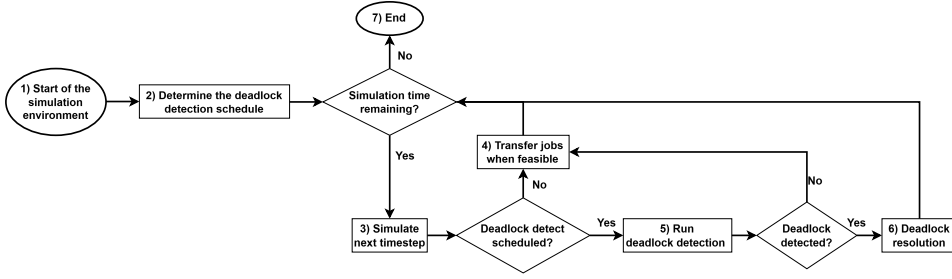
Figure 6.7: Flow diagram illustrating the simulation process, including deadlock detection and resolution.
