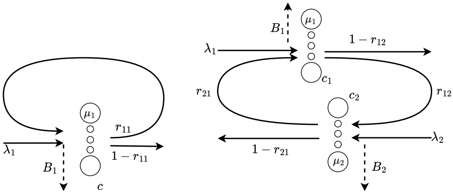
Figure 6.3: One- and two-node queueing network with ASB and potential deadlocks.
