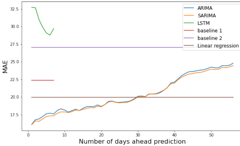
Figure 7.24: The MAE error when forecasting telephone.
