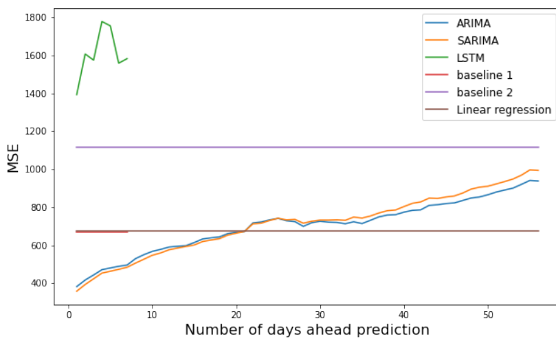
Figure 7.23: The MSE error when forecasting chat.
