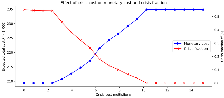
Figure 4.9: Effect of decreasing the fraction of patients experiencing a crisis (red) on the total expected cost (blue) using the crisis cost multiplier \alpha .
