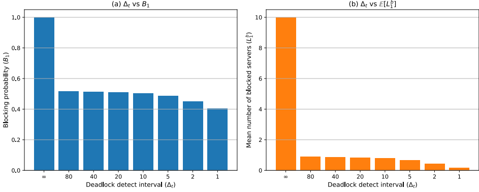
Figure 6.9: The impact of \Delta_t on B_1 and E[L_1^b] in the simulation of a two-node system.
