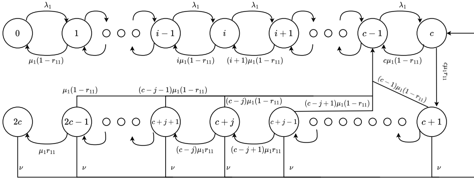
Figure 6.4: Continuous-time Markov chain of one-node network with ASB and deadlock resolve.
