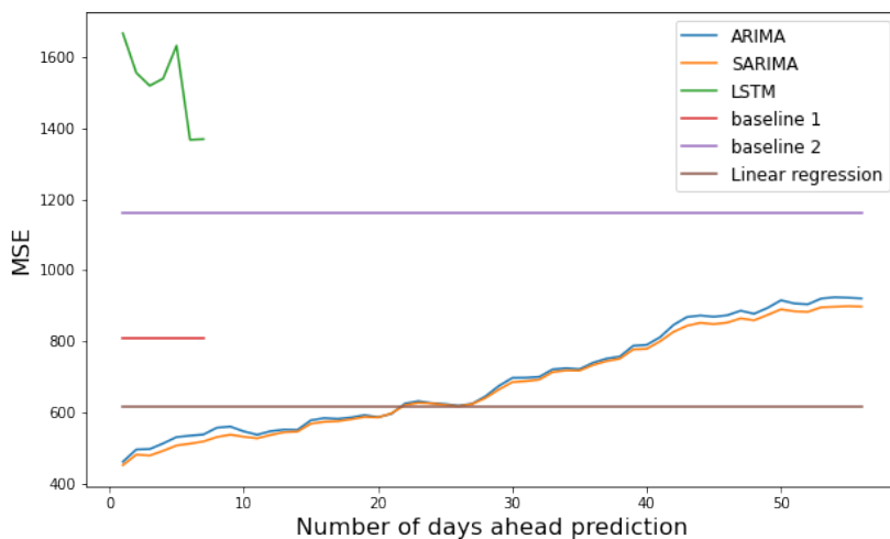
Figure 7.22: The MSE error when forecasting telephone.
